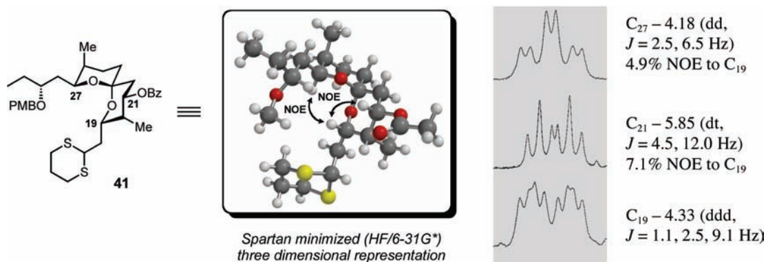
Figure 3. NOE and Coupling Constant Analysis of the Spiroketal.
